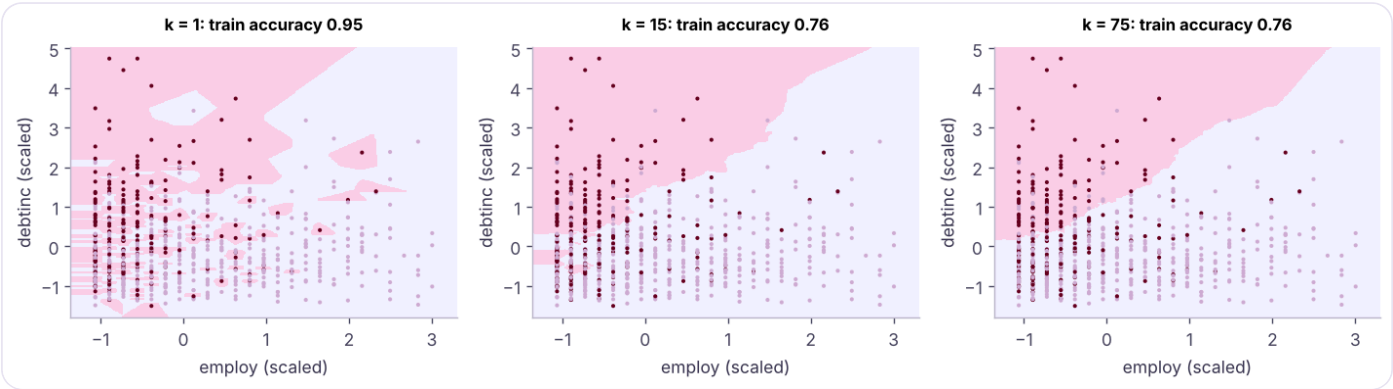
Decision boundaries for k = 1, 15 and 75 on two standardised features: small k overfits with jagged islands; large k oversmooths.
