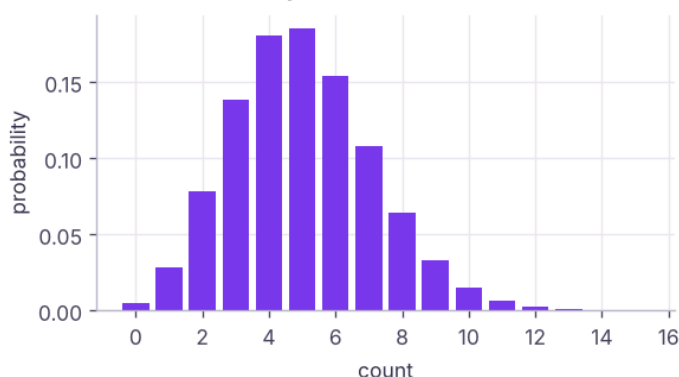
Binomial( n=50 , p=0.1 )
